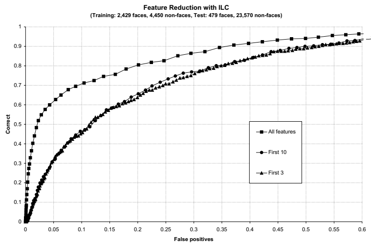
Figure 5: ROC curves for SVMs with 2nd-degree polynomial kernel trained on feature sets generated by ILC.
